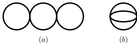
Figure 4. Three-loop vacuum diagrams.
